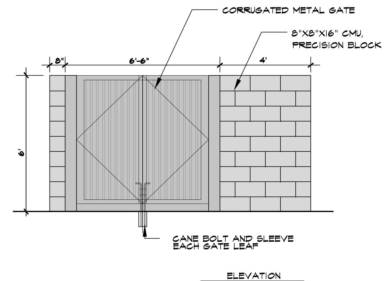
TRASH ENCLOSURE DETAIL SCALE: NTS
