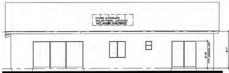
REAR ELEVATION SCALE=1/4"
