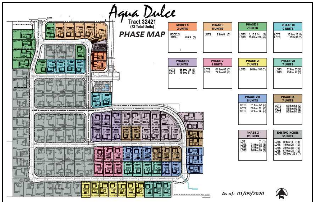
Figure 1: Phasing Plan
