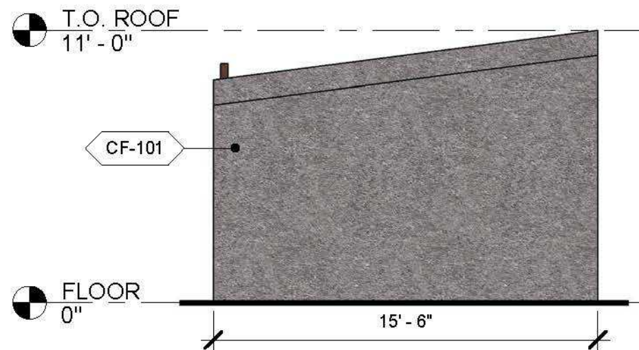
② LEFT ELEVATION - COMMUNAL MUD BATH 3/16" = 1'-0"
