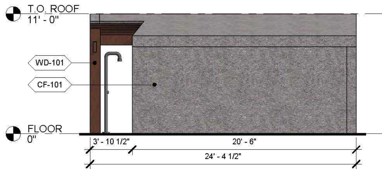
③ REAR ELEVATION - COMMUNAL MUD BATH 3/16" = 1'-0"
