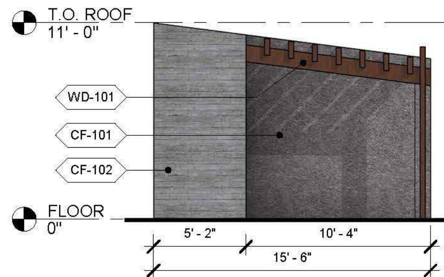
④ RIGHT ELEVATION - COMMUNAL MUD BATH 3/16" = 1'-0"
