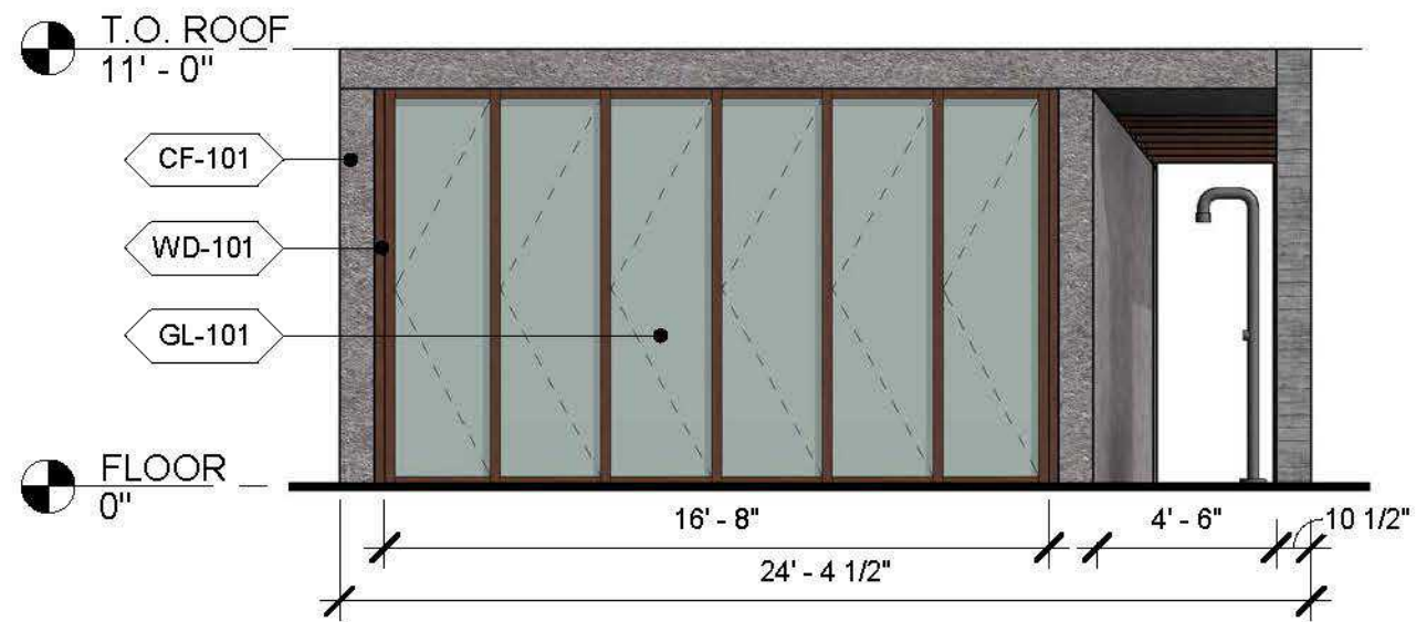
① FRONT ELEVATION - COMMUNAL MUD BATH 3/16" = 1'-0"
