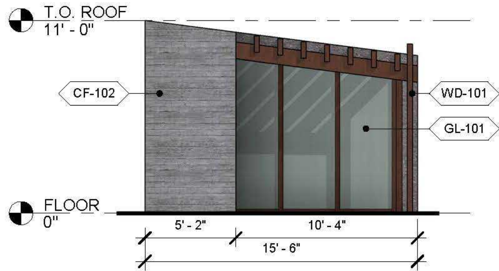
① FRONT ELEVATION - DOUBLE DRY TREATMENT ROOM 3/16" = 1'-0"
