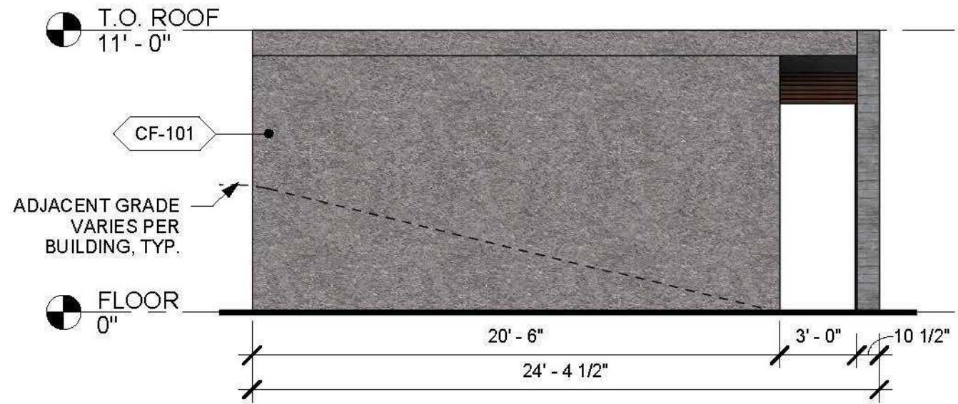
② LEFT ELEVATION - DOUBLE DRY TREATMENT ROOM 3/16" = 1'-0"
