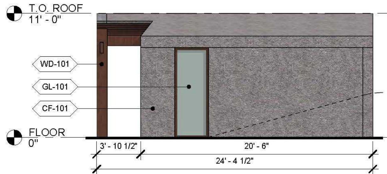
④ RIGHT ELEVATION - DOUBLE DRY TREATMENT ROOM 3/16" = 1'-0"
