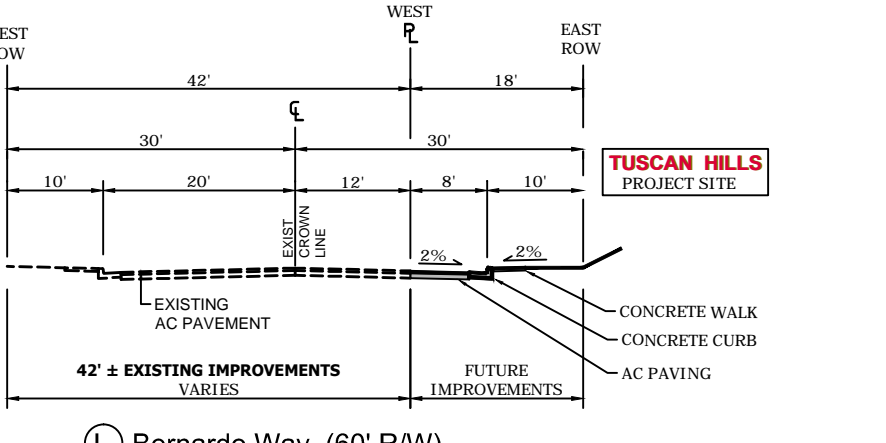
Bernardo Way (60' RW) Public Street
