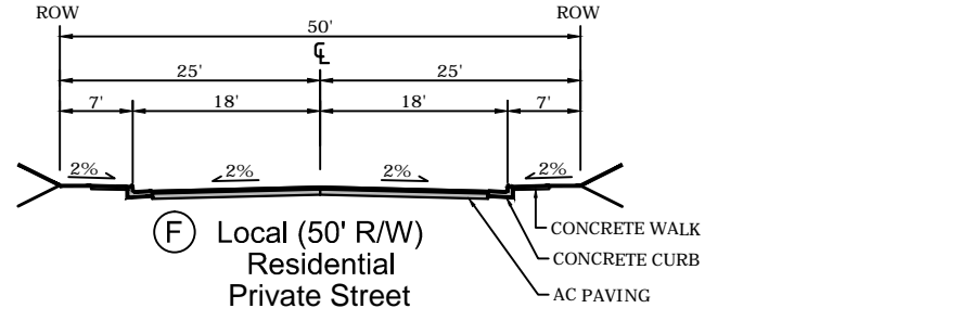
Local (50' RW) Residential Private Street
