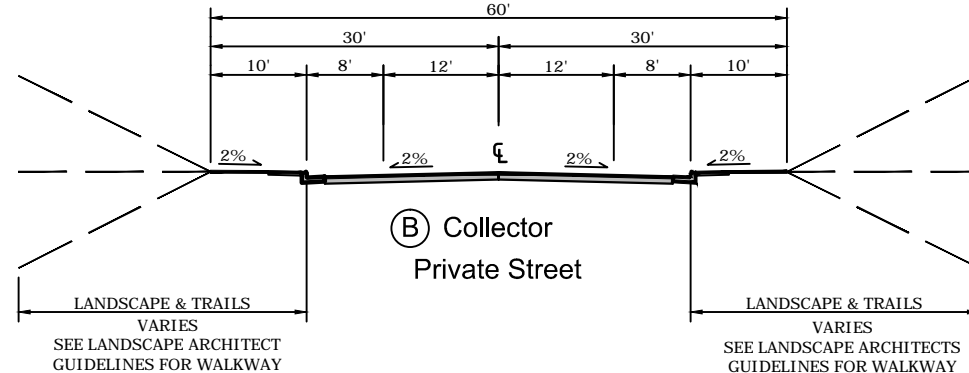
Collector Private Street
