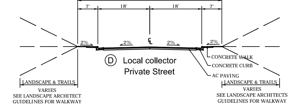
Local collector Private Street
