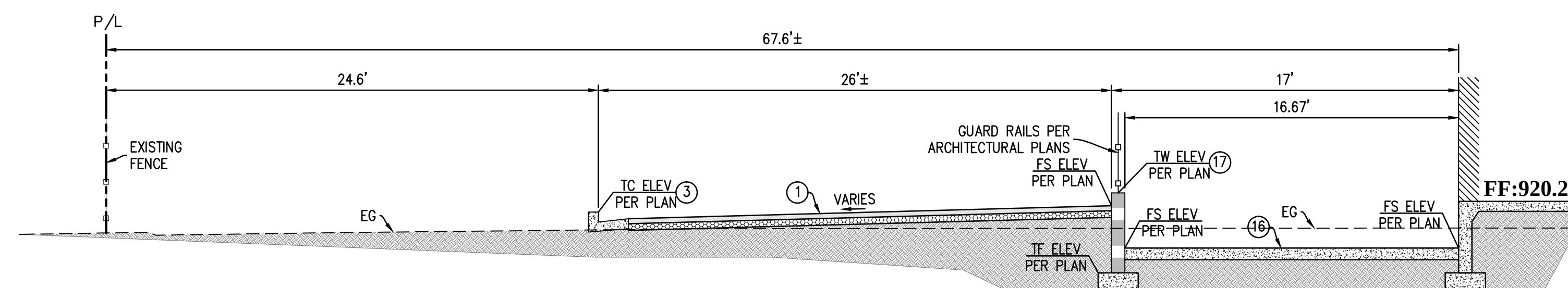
SECTION F-F SCALE: 1"=5'
