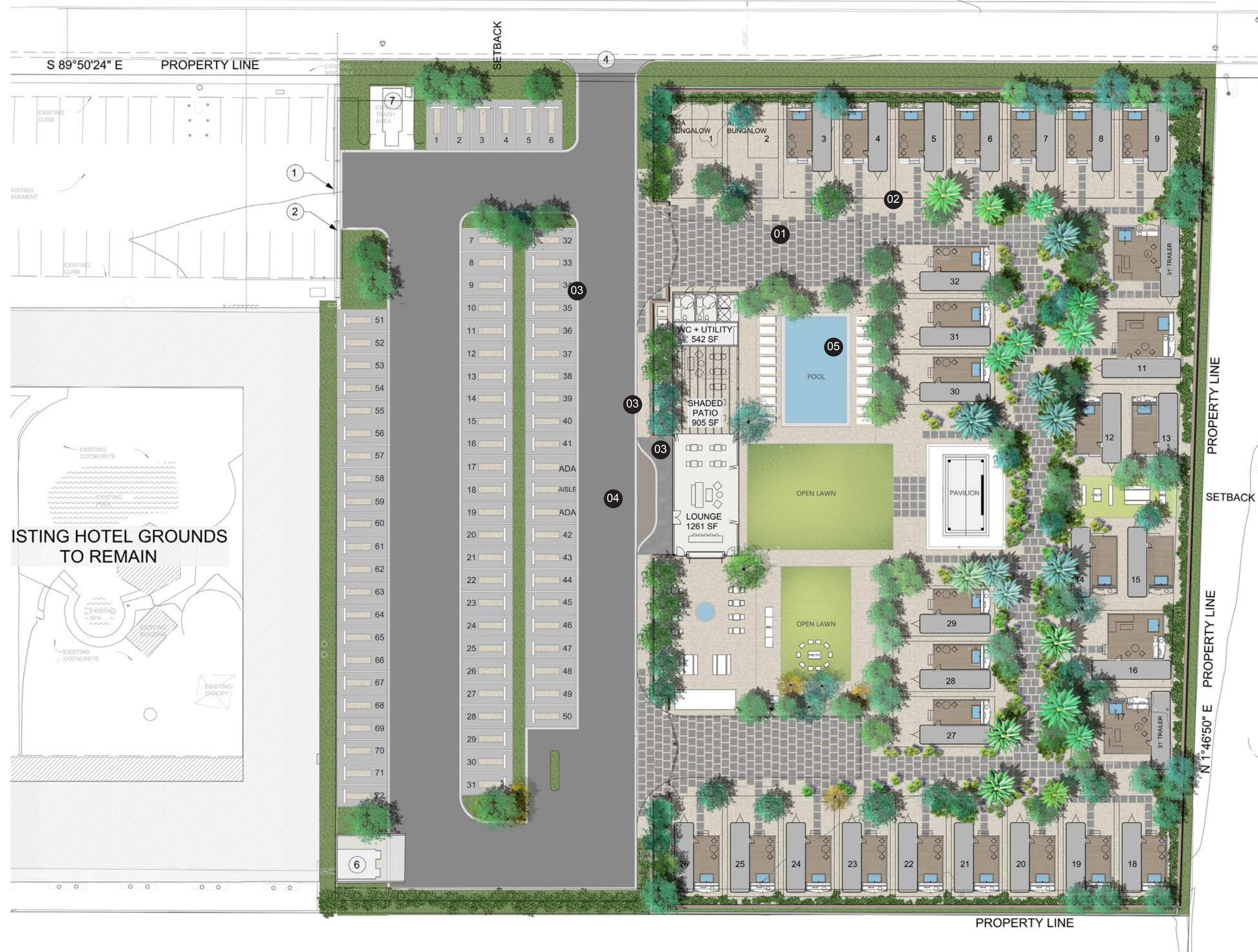
01 800X800MM CONCRETE STEPPING STONE 02 GRAVEL
