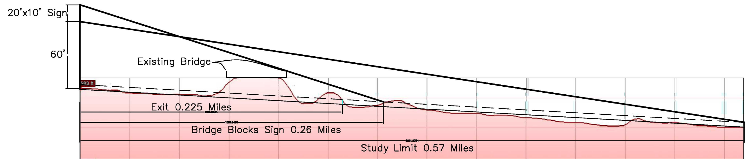
Westbound Sign Visibility Profile
