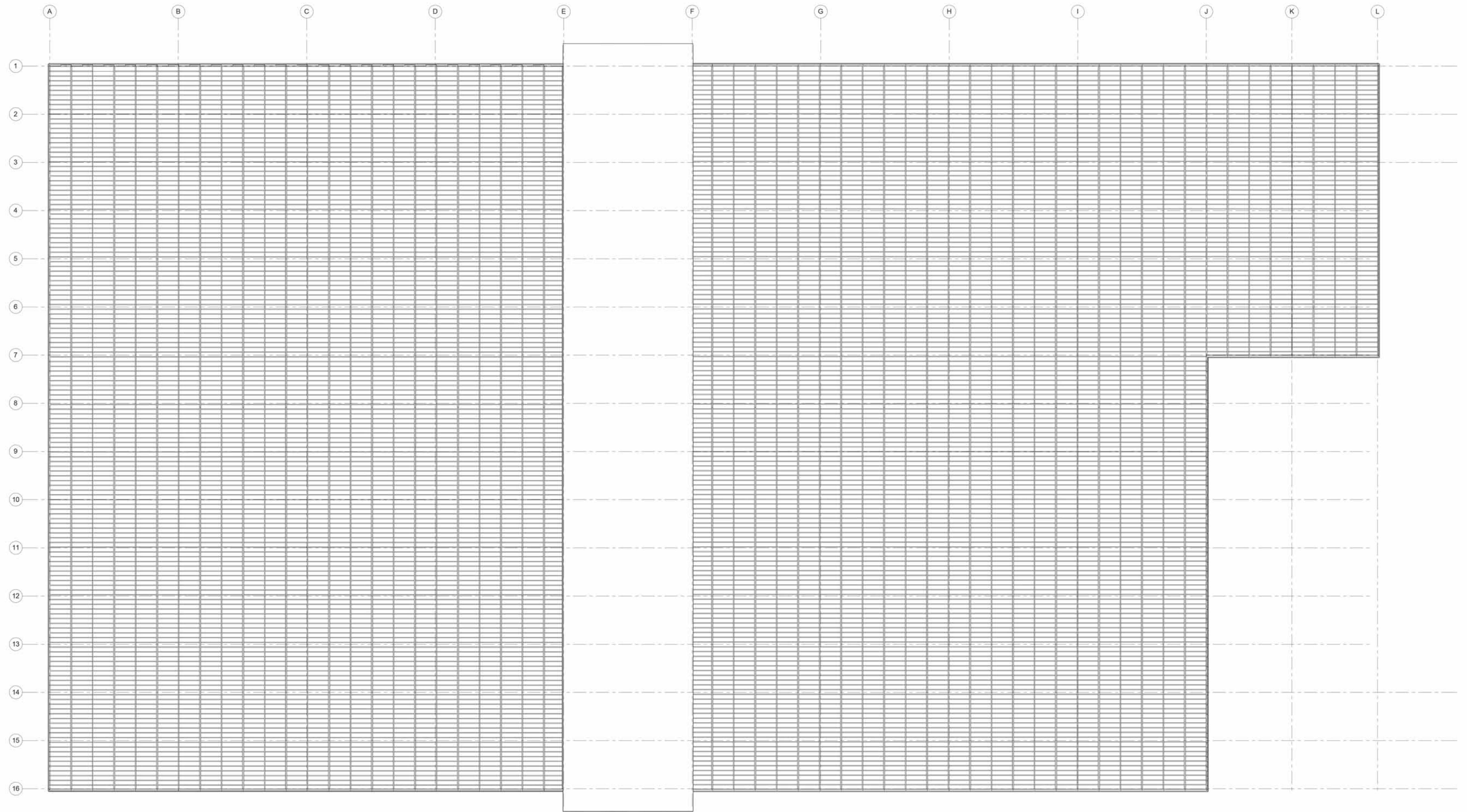
ROOF PLAN ELEV: +18.5 m [60'-8"] 1" = 20'
