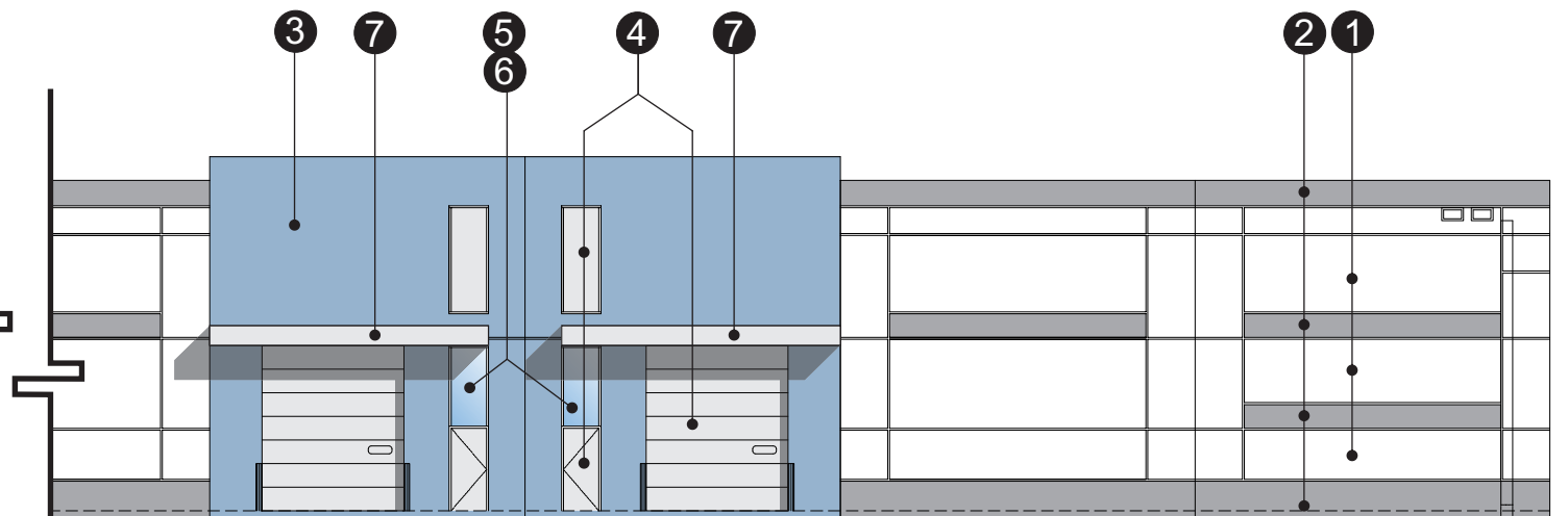
Enlarged View of East Elevation
