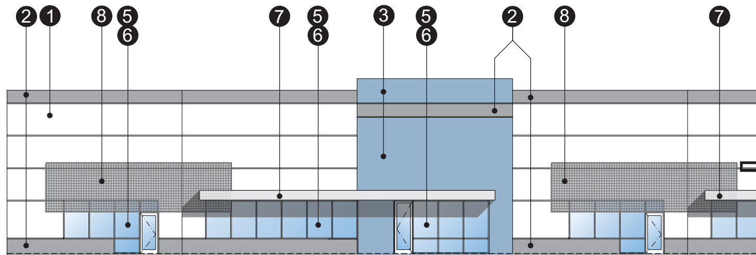
Enlarged View of West Elevation
