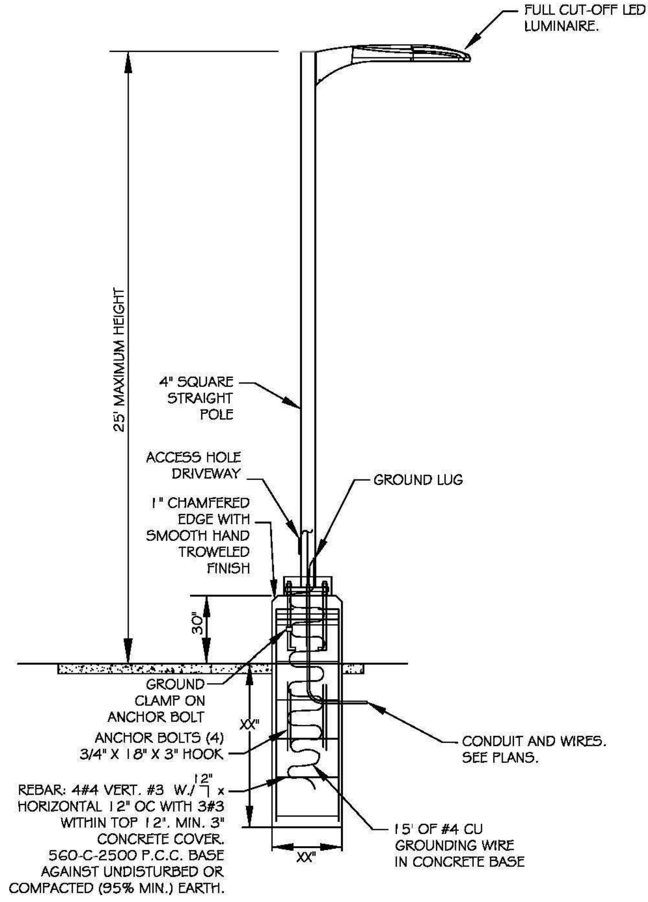
NO SCALE A TYPE 'A' & 'B' STREET LIGHT INSTALLATION DETAIL
