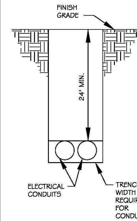
NO SCALE D TRENCH AND CONDUIT INSTALLATION DETAIL
