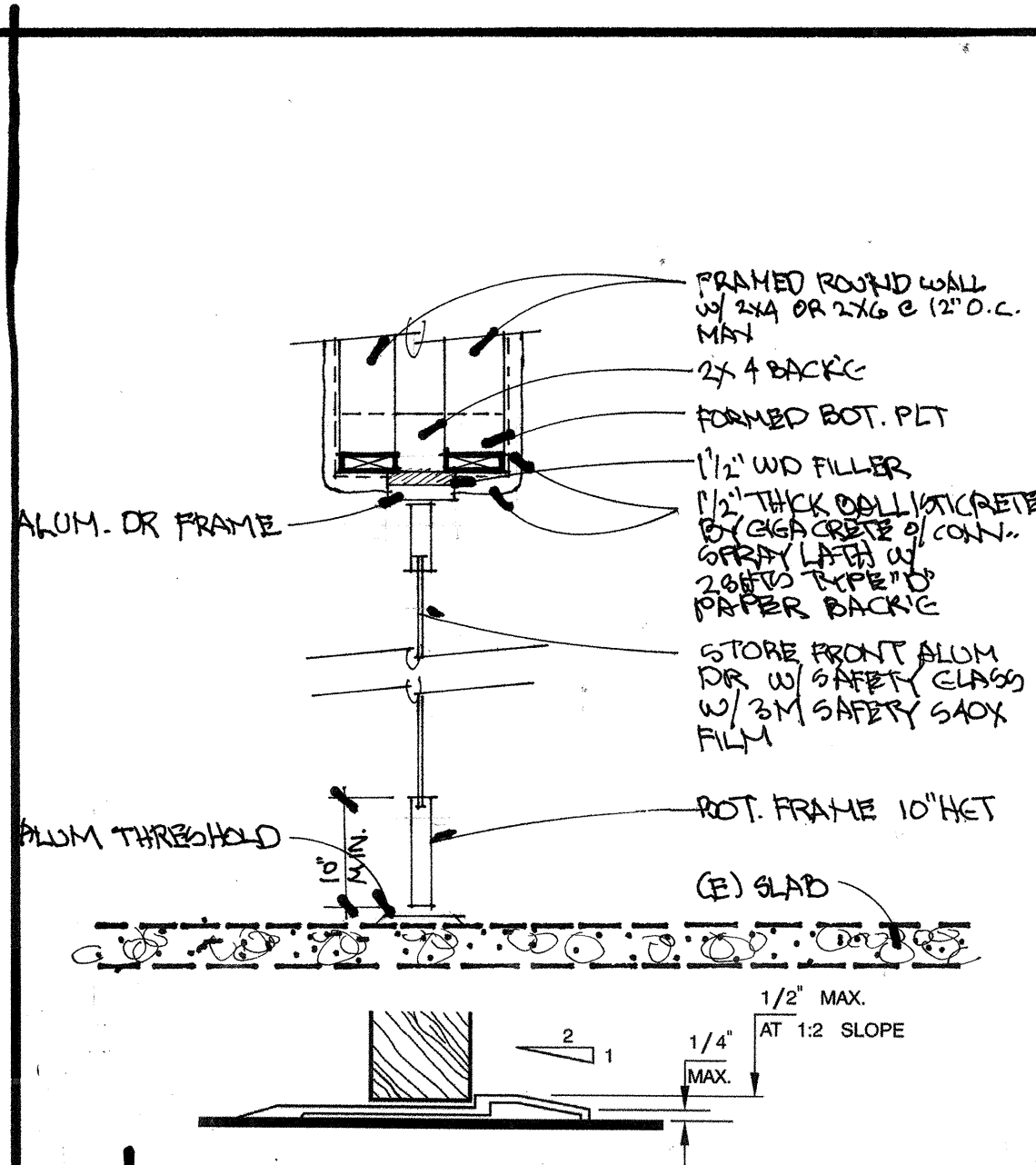
4 dbi round ballistic plaster wall & dr scale: 3/4" = 1'-0"
