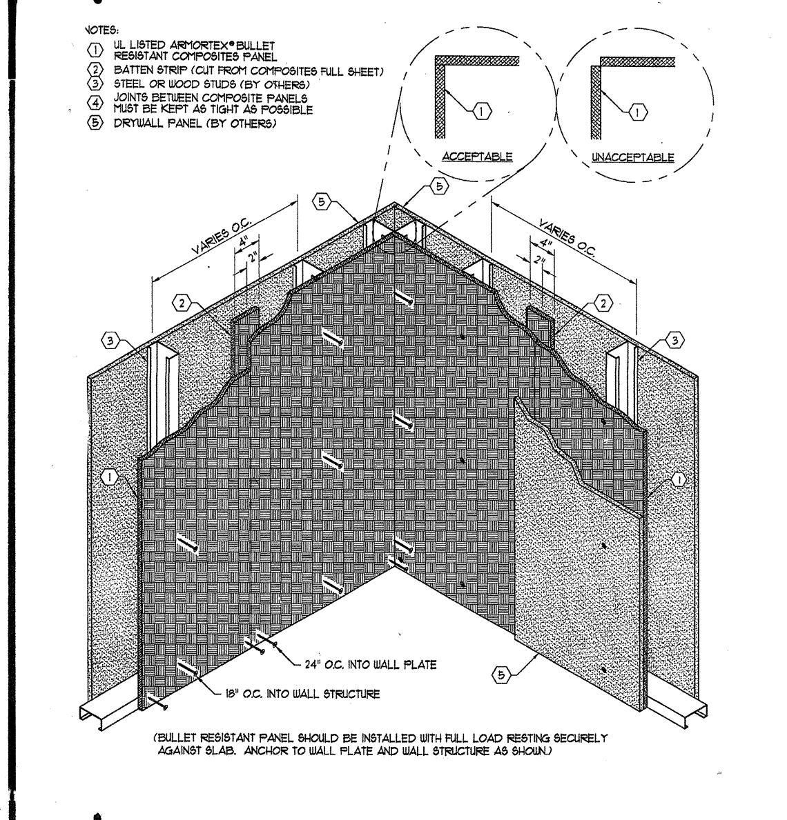
9 ballistic fiberboard construction no scale
