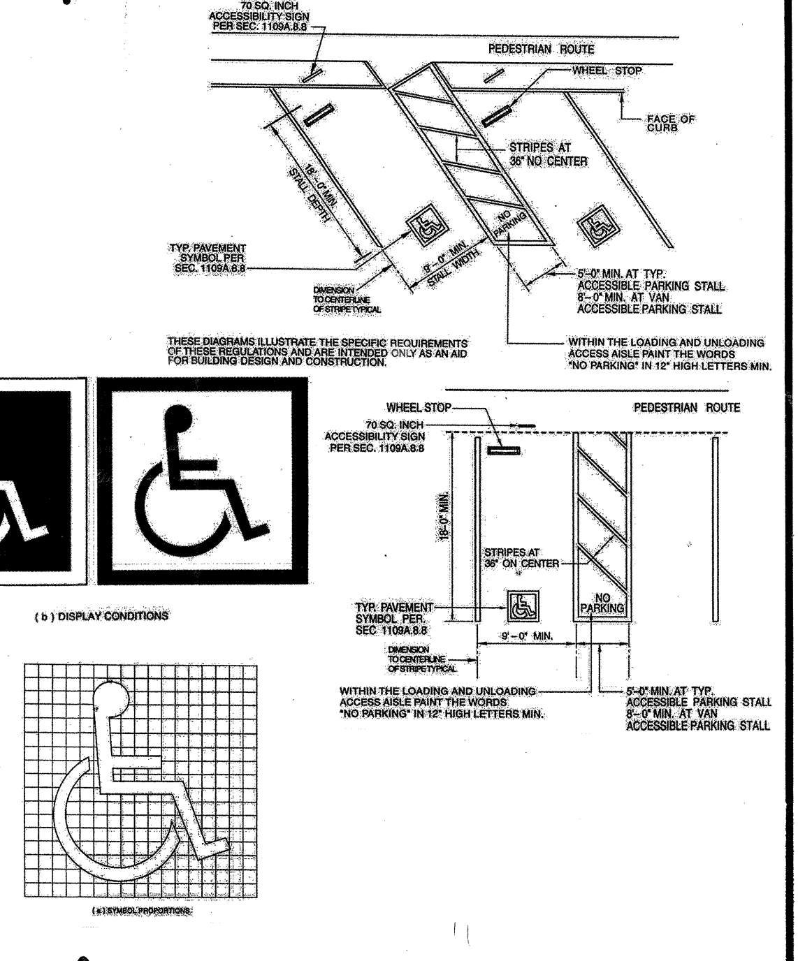
11 accessible parking no scale
