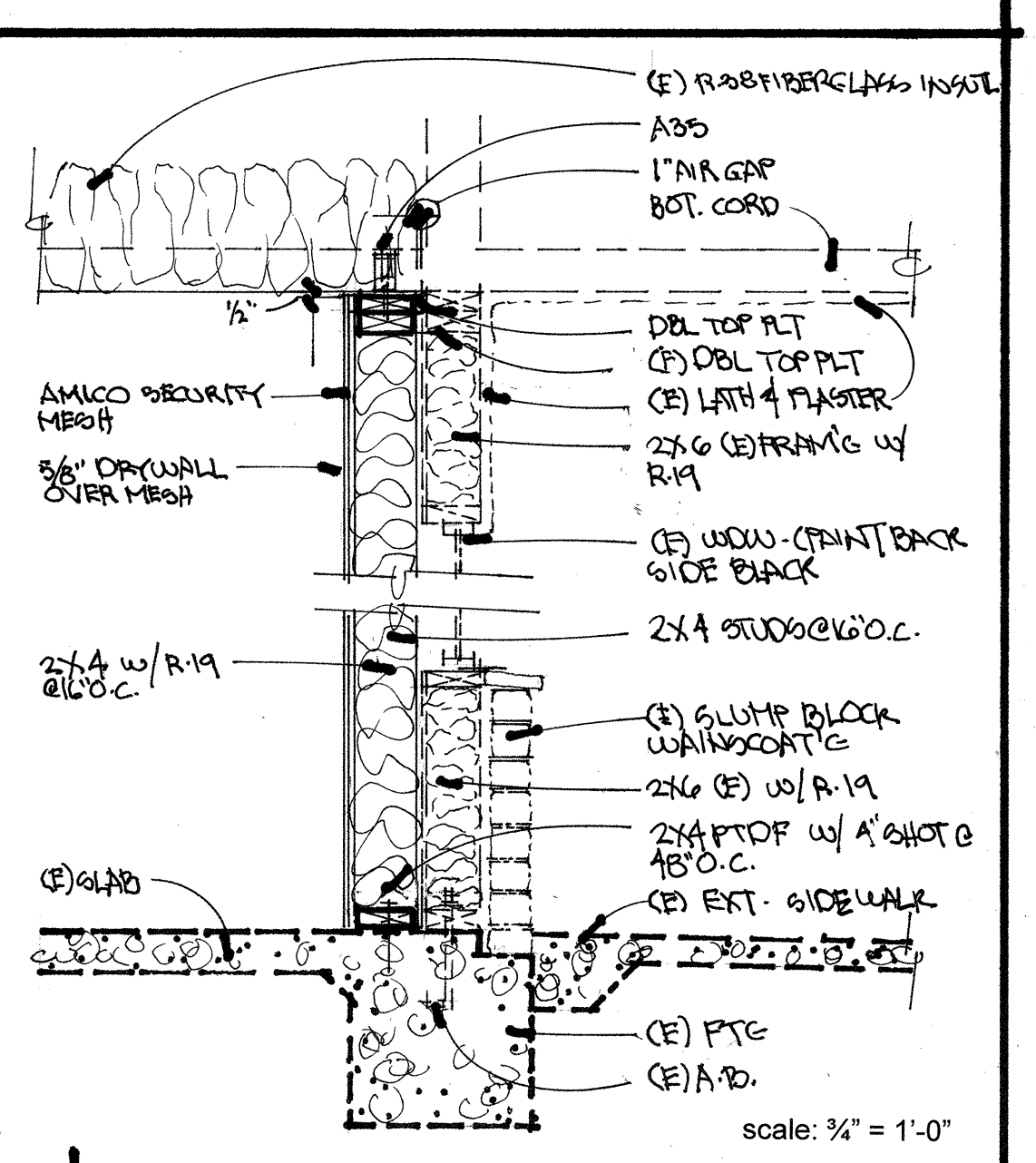
1 perimeter ballistic plaster/security mesh wall
