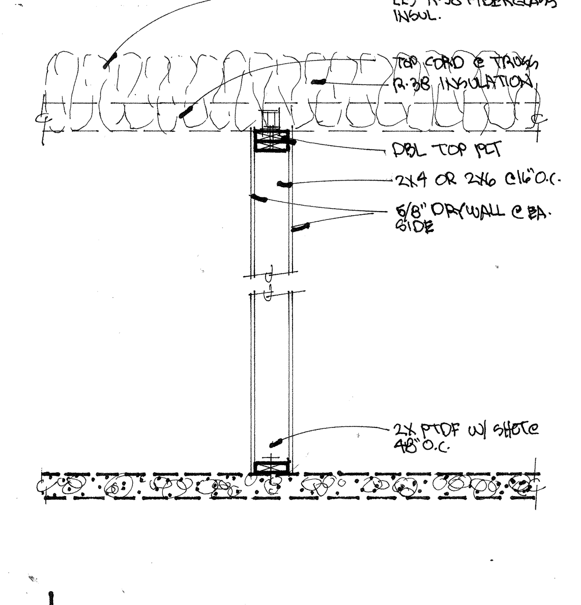
8 partition wall scale: 3/4" = 1'-0"
