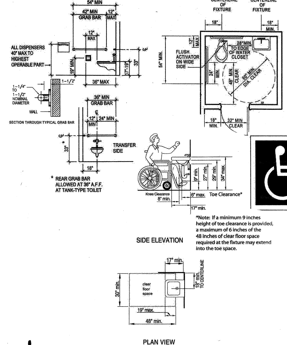
12 accessible restrooms no scale
