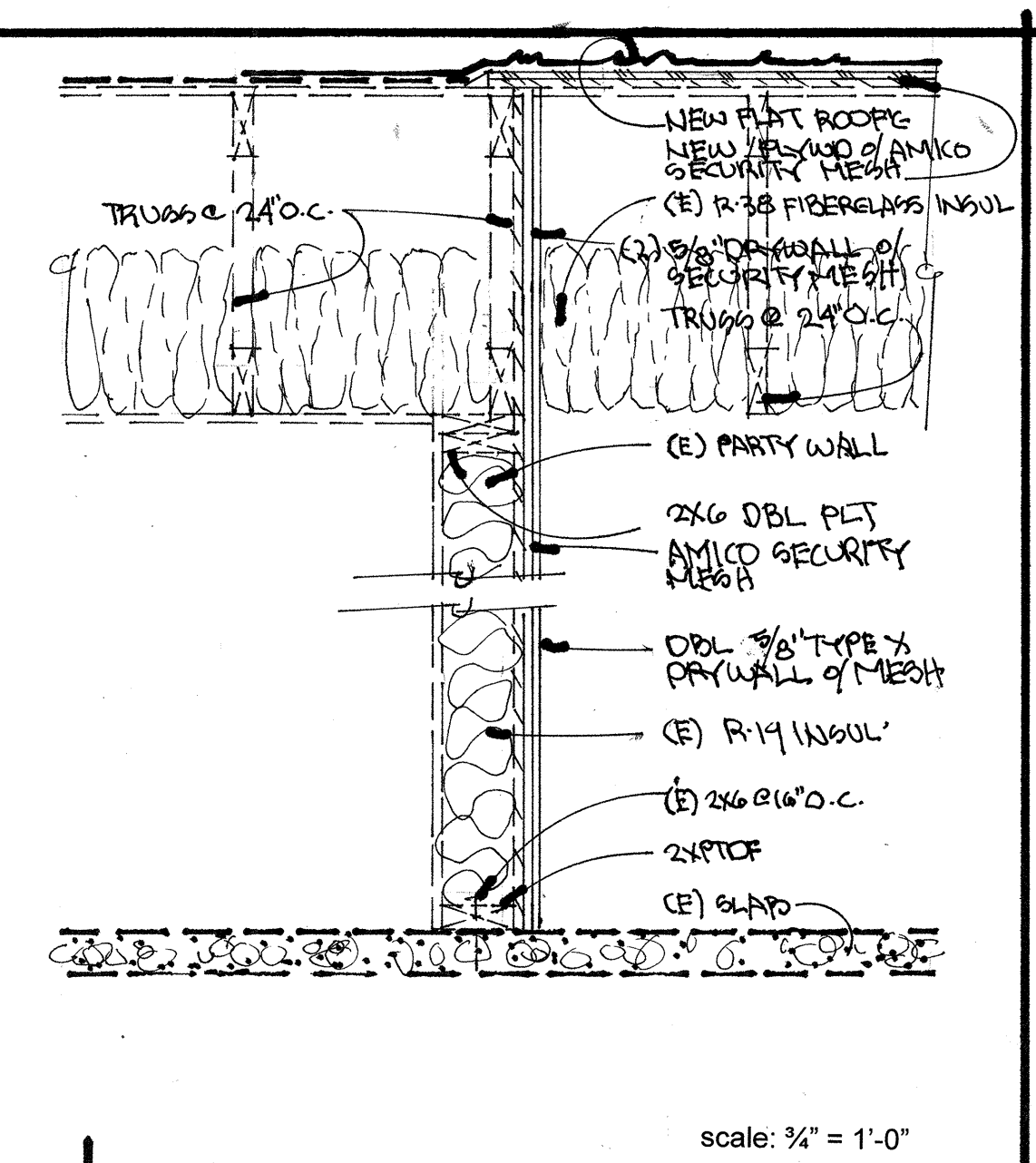
2 party ballistic fiberboard/security mesh wall
