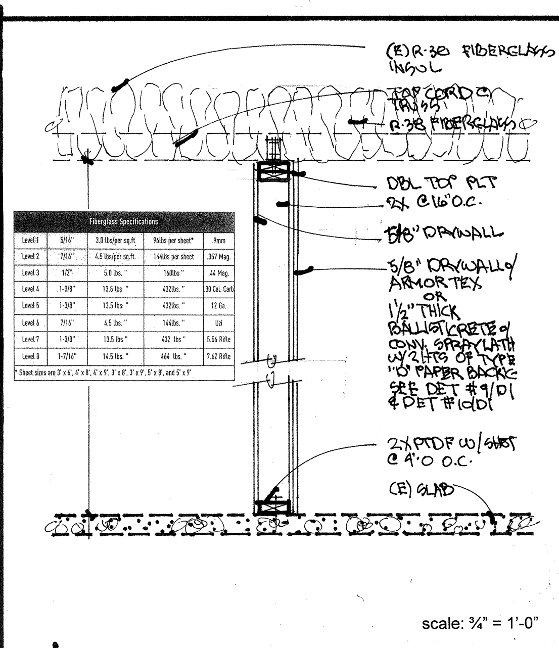
5 partition ballistic (plaster or fiberboard) wall
