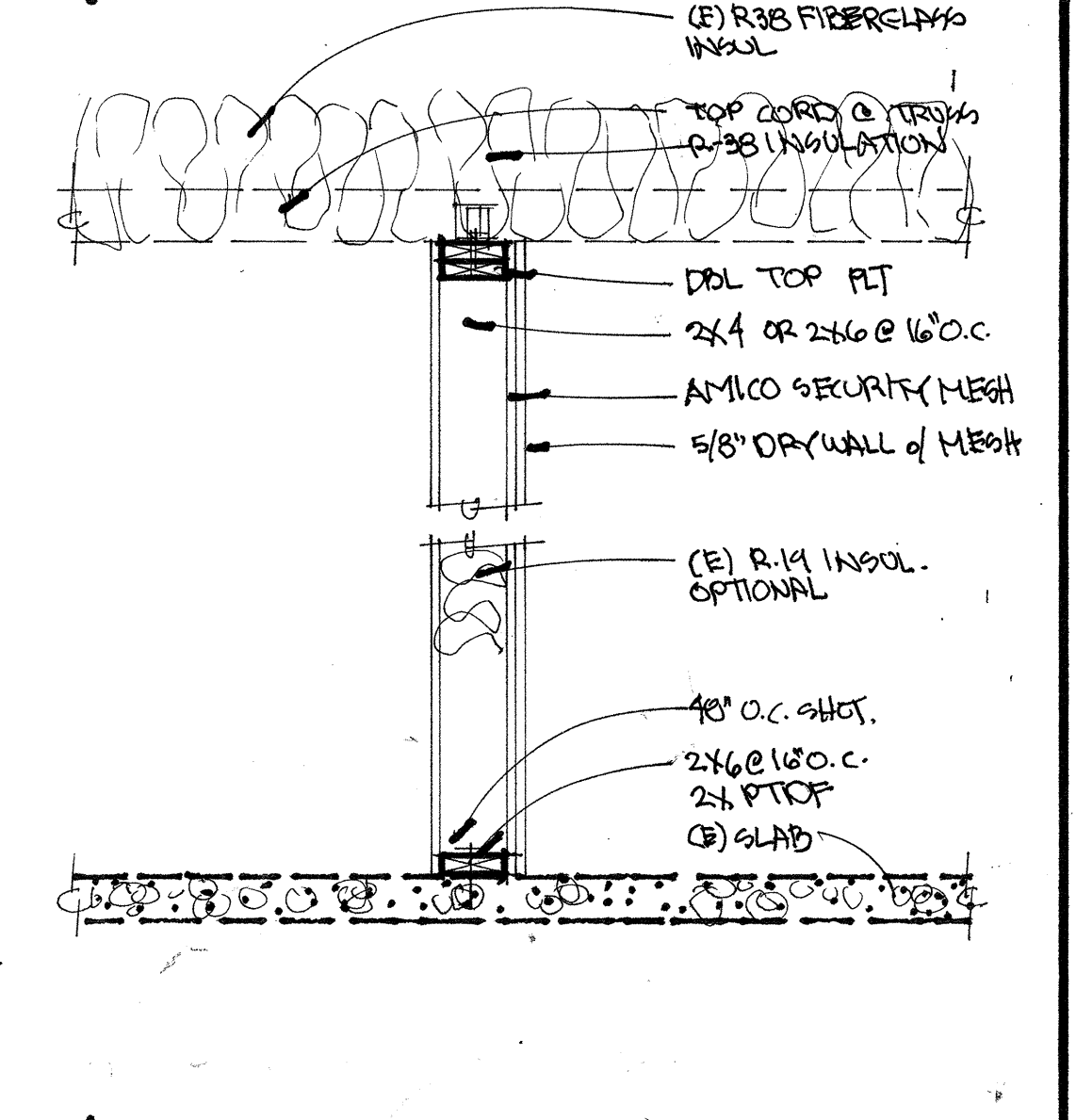
7 partition security mesh wall scale: 3/4" = 1'-0"
