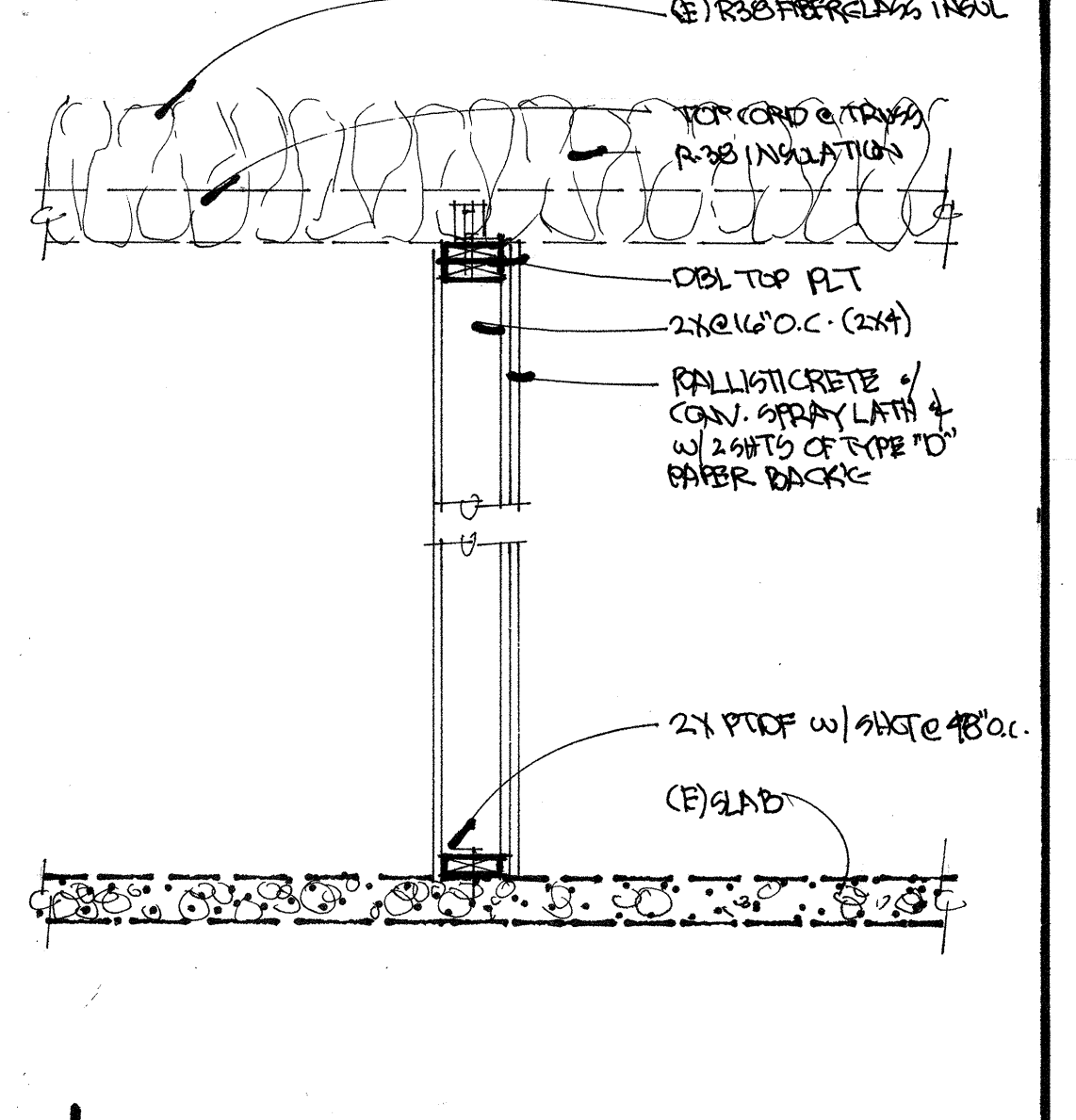
6 partition ballistic plaster wall scale: 3/4" = 1'-0"
